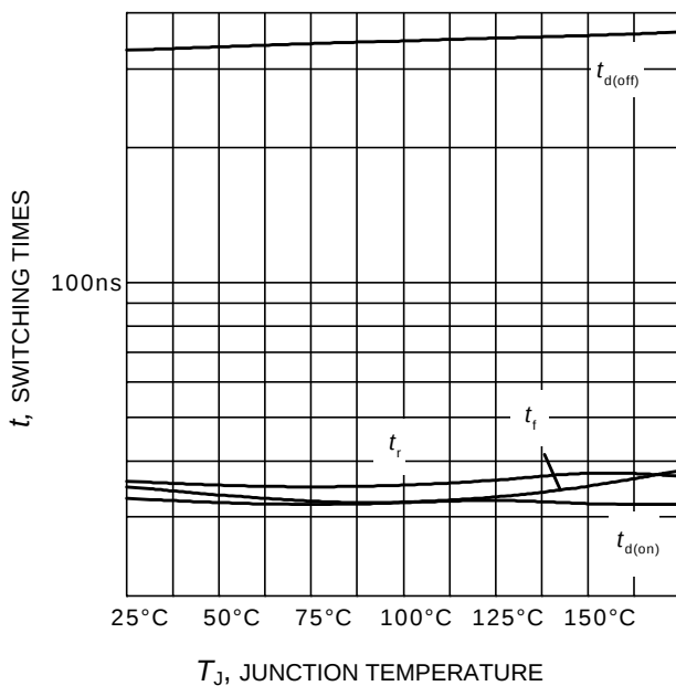
Figure 11. Typical switching times as a function of junction temperature (inductive load, V_{CE}=400\text{V} , V_{GE}=0/15\text{V} , I_C=75\text{A} , r_G=5\Omega , Dynamic test circuit in Figure E)
