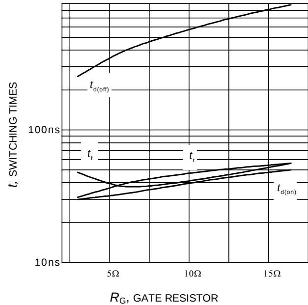
Figure 10. Typical switching times as a function of gate resistor (inductive load, T_J=175^\circ\text{C} , V_{CE}=400\text{V} , V_{GE}=0/15\text{V} , I_C=75\text{A} , Dynamic test circuit in Figure E)
