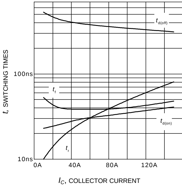
Figure 9. Typical switching times as a function of collector current (inductive load, T_J=175^\circ\text{C} , V_{CE}=400\text{V} , V_{GE}=0/15\text{V} , r_G=5\Omega , Dynamic test circuit in Figure E)
